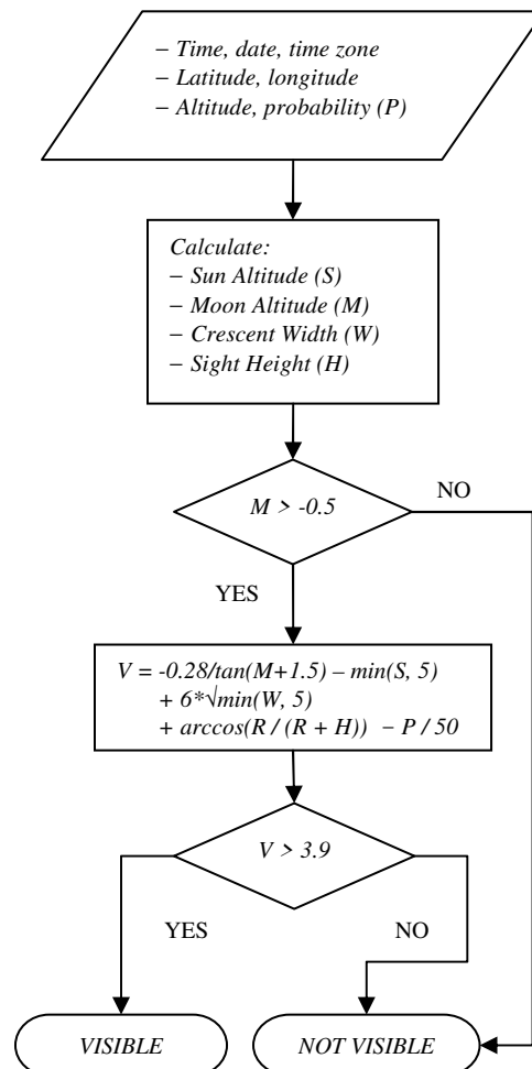
Figure 10 – Flowchart of Proposed Visibility Algorithm
